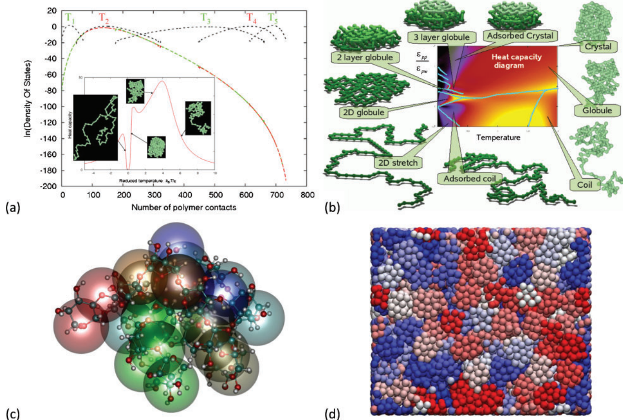
4 Examples of mesoscale modelling in coarse grained systems a reconstruction of DOS for a lattice chain polymer by histogram reweighting, with heat capacity versus reduced temperature shown as inset, and b heat capacity for lattice chain adsorbed on flat surface, showing surface induced crystallisation and multilayer coil-globule transitions, c off-lattice representation of oligosaccharide (larger semitransparent spheres) superimposed on corresponding atomic configuration and d model for granular material composed of assembly of cohesive spheres (those in each granule coloured identically) For a video of figure 4d, please go to Supplementary Material 1 http://dx.doi.org/10.1179/1743280410Y.000000002.S1
