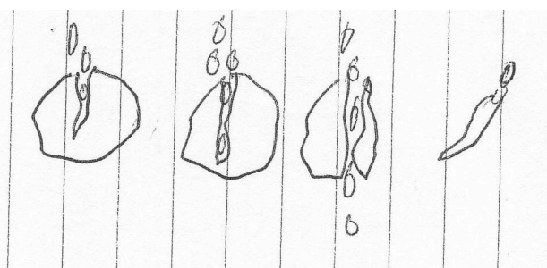
Sugar being broken down by water
