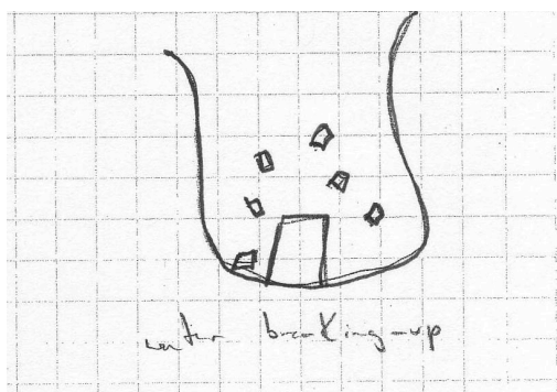
A sugar crystal being broken down by water. I9Y11
