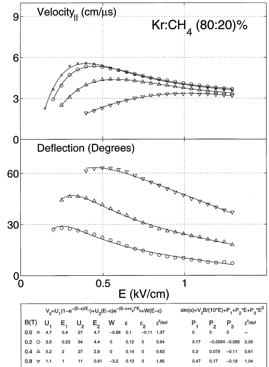
Fig. 6. For Kr: CH 4 (80 : 20)%, more parameters are needed for a good description.
