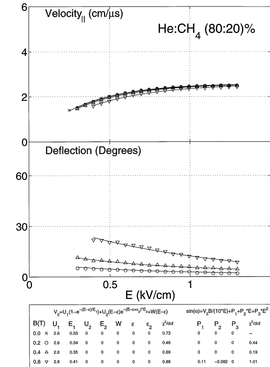
Fig. 5. He: CH 4 (80 : 20)%. An empirical fit overlaying data with the formula and parameters given below.
