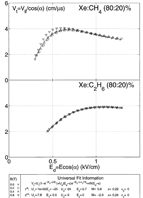
Fig. 9. For Xe : CH 4 (80 : 20)%, velocities are higher than expected at B = 0.8 T.
