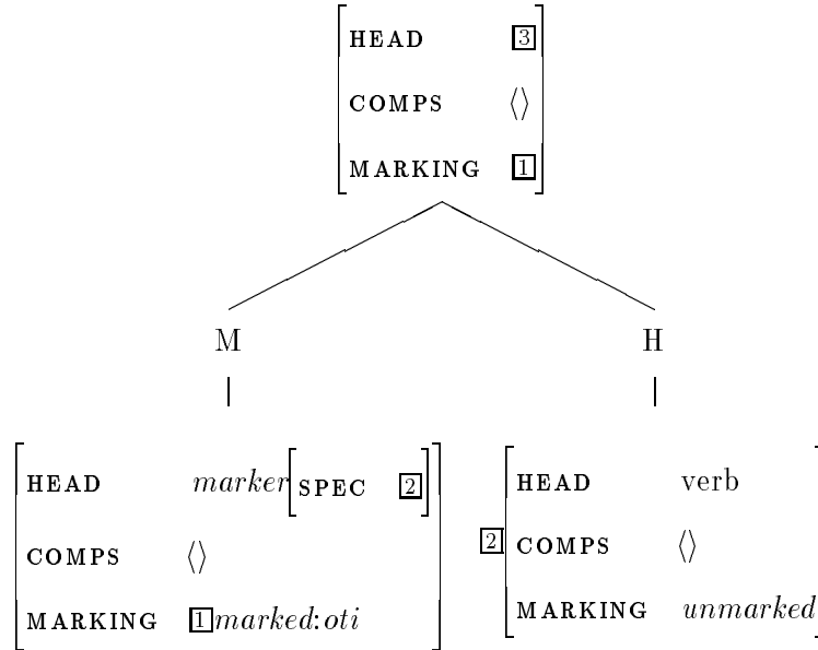
(4.32) HEAD-MARKER-ID-SCHEMA
